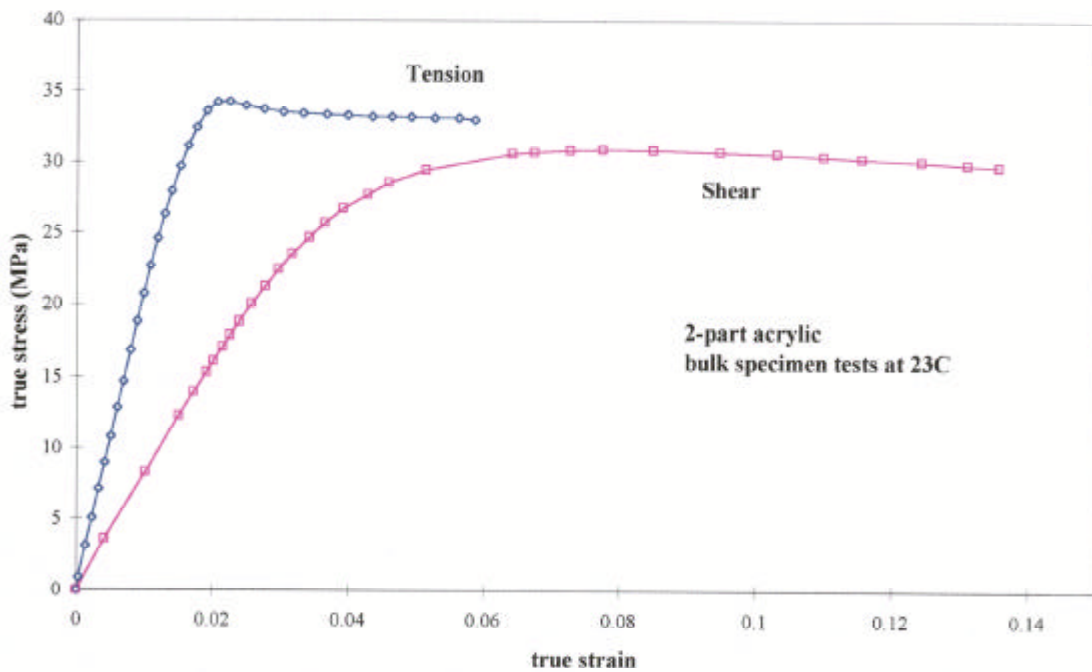
Figure 3. Stress/strain curves obtained under uniaxial tension and pure shear for a toughened acrylic adhesive.
