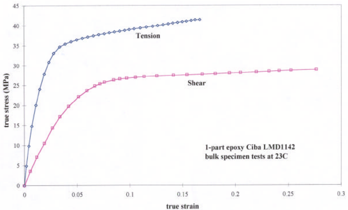
Figure 1. Stress/strain curves obtained under uniaxial tension and pure shear for a toughened epoxy adhesive.
