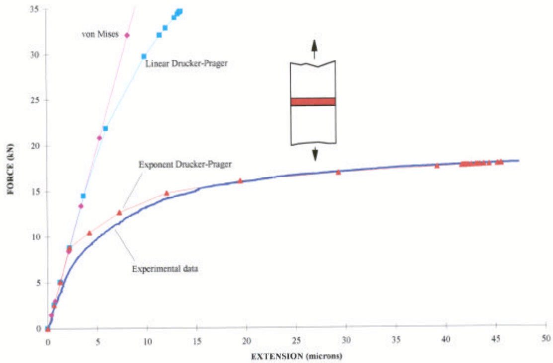
Figure 2: Comparison of measured and calculated force versus extension curves for a butt-joint loaded in tension. The extension is determined between points on each adherend located 3 mm from the bond. The bond thickness is 0.5 mm and the adherends are steel.
